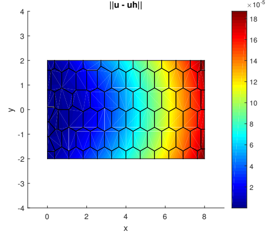
(b) Parabolic beam - FEM
