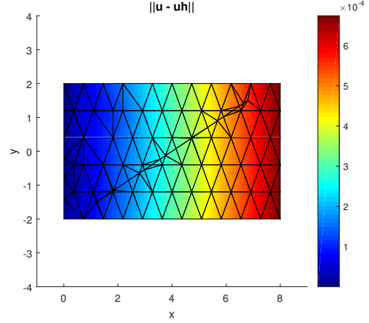
(b) Breaking with a diagonal line - FEM
