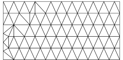
(b) Mesh for the parabolic beam tests - FEM
