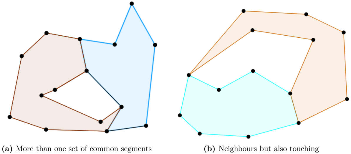
Figure 5.6: Unmergeable polygon dispositions
