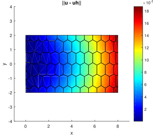
(a) Parabolic beam - VEM
