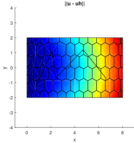
(a) Breaking with a zigzagging sequence - VEM
