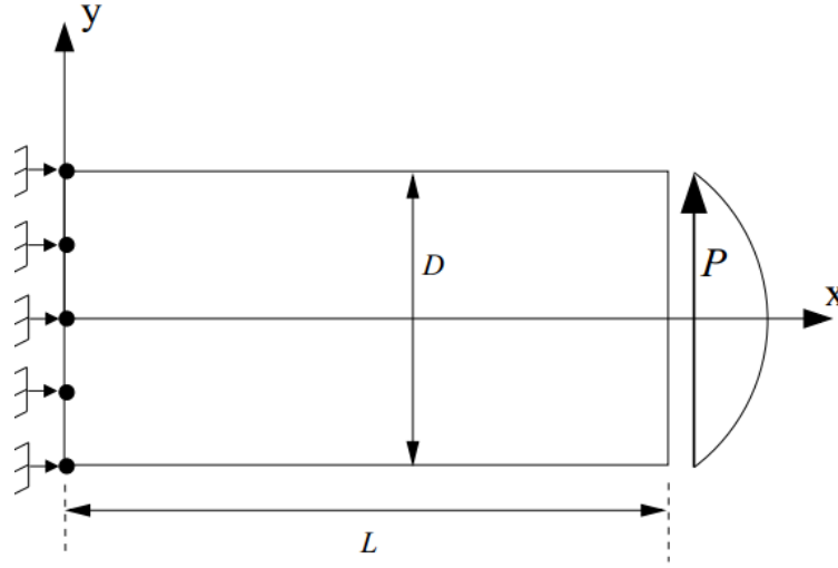
Figure 4.11: Parabolic beam test
