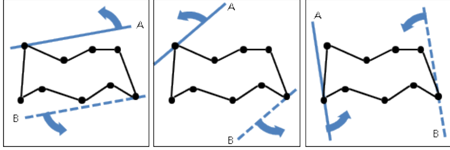
Figure 2.8: Rotating calipers algorithm
