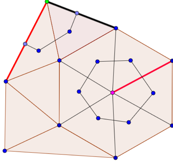
Figure 5.2: Both stop conditions for Voronoi cells
