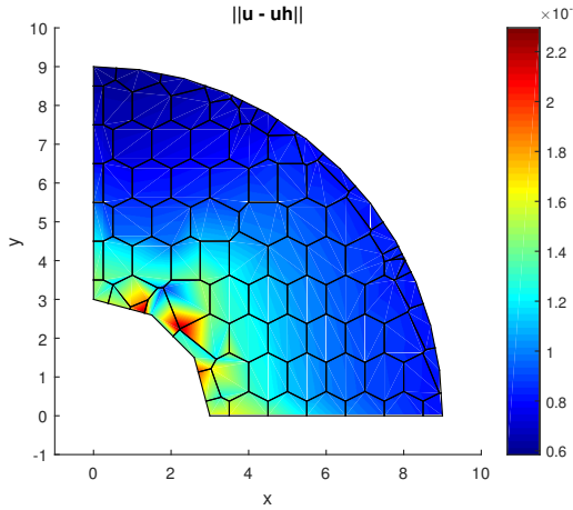
(c) Pressurized cylinder - VEM
