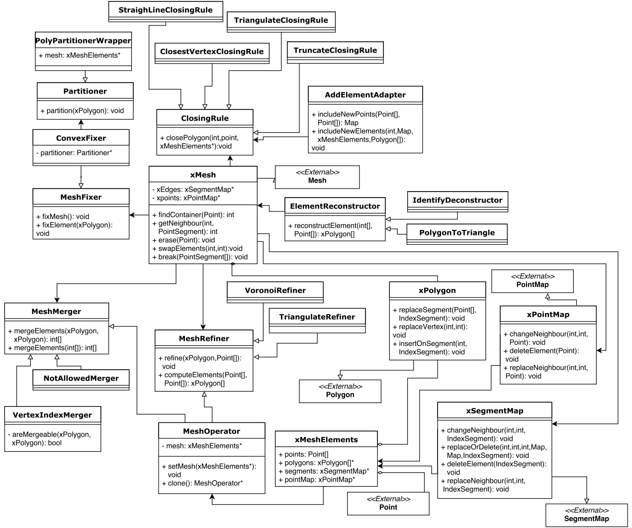
Figure 4.10: UML class diagram of modifiable meshes library
