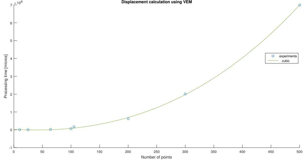
Figure 6.2: Results of time experiments on the Virtual Element Method library
