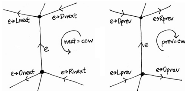
Figure 2.6: Winged-edge data structure
