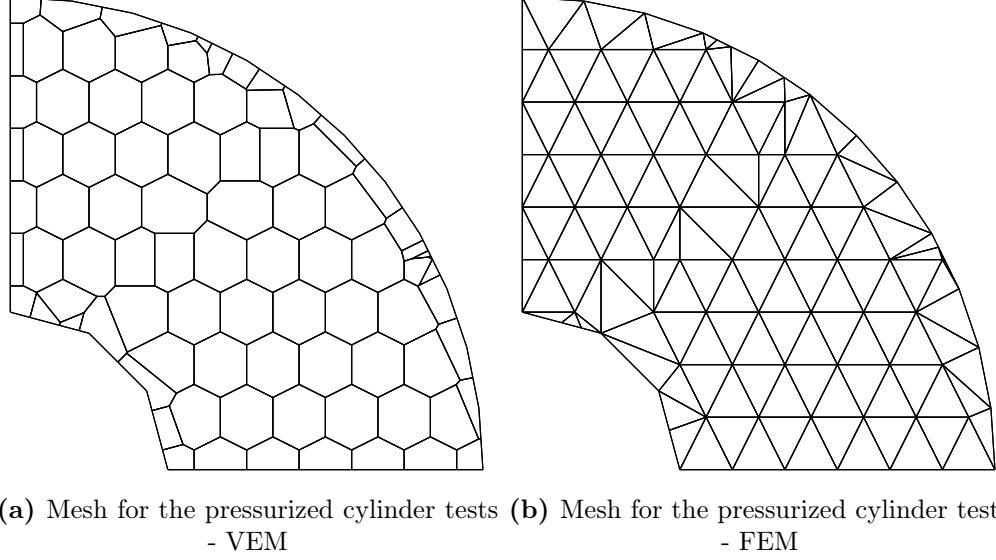
Figure 6.9: Meshes for the pressurized cylinder tests, for both methods
