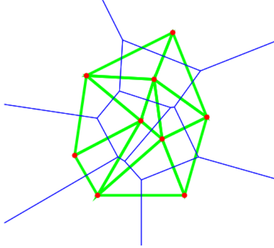
Figure 2.3: Delaunay-Voronoi duality
