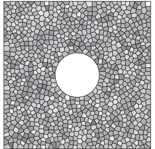
(b) Quasi-random mesh
