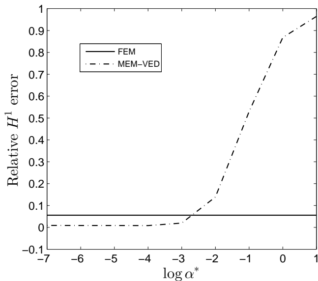
Figure 14: Pressurized thick-walled cylinder problem. Sensitivity analysis of \alpha^* in the H^1 seminorm.
